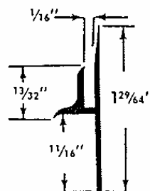
467* FOR 1/4" MATERIAL
