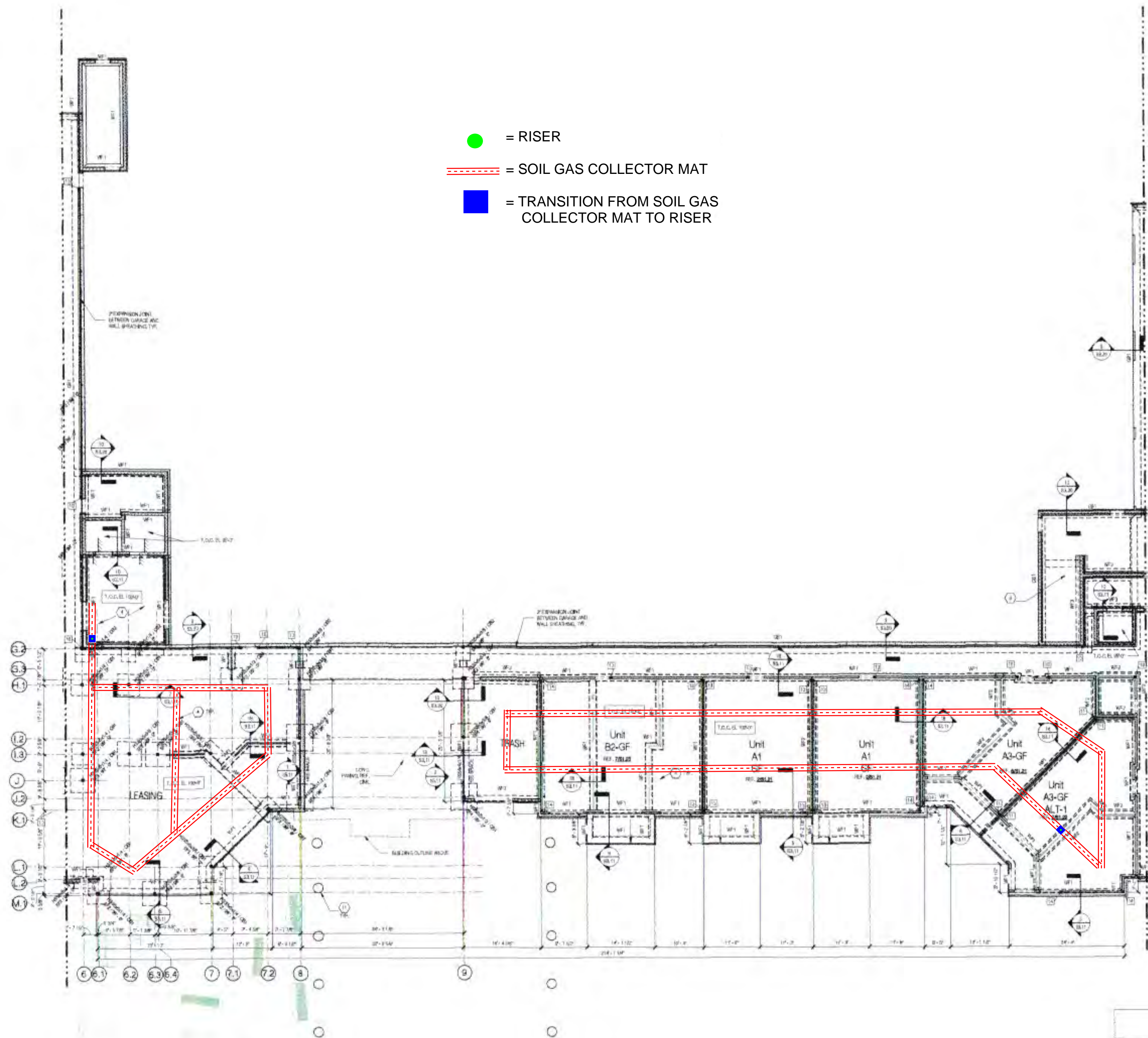
1 FOUNDATION PLAN - AREA B
