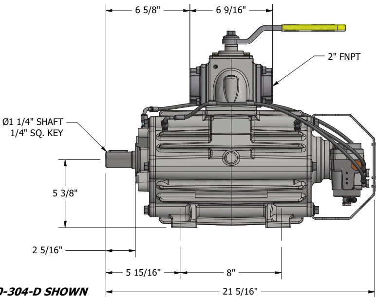
110-304-D SHOWN (CW PUMP)
