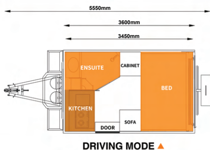
DRIVING MODE ▲
