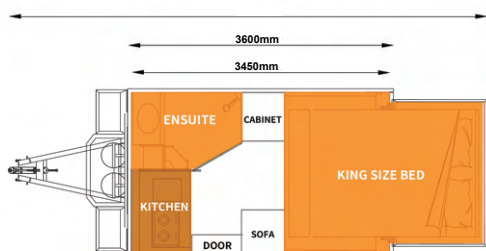
PARKING MODE ▲
