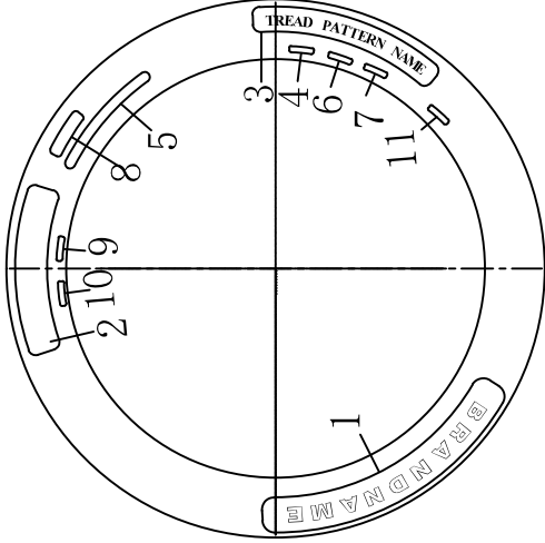
UPPER MOULD
