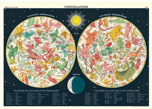
Constellations 2
