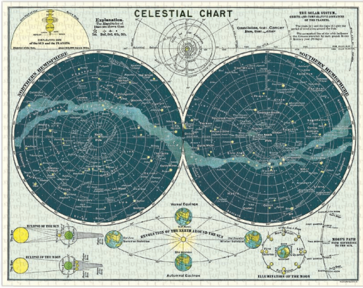
Celestial
