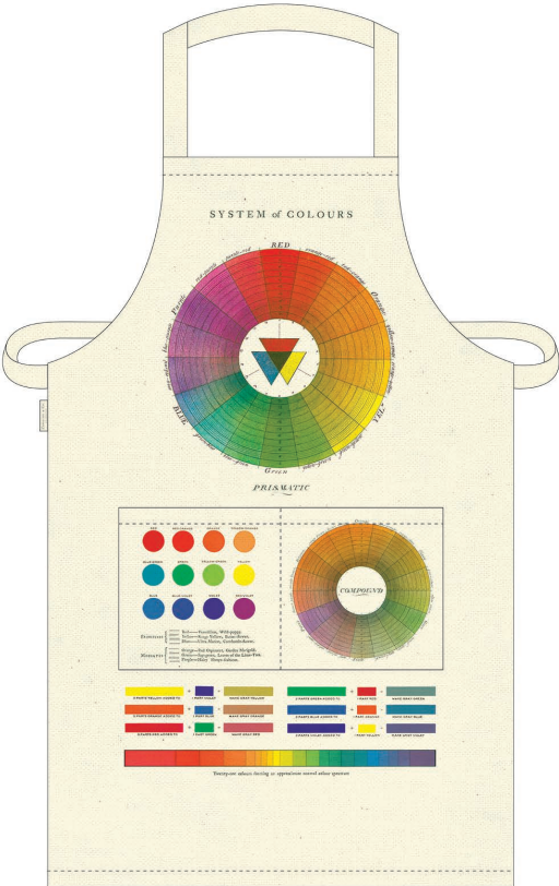
Color Wheel
