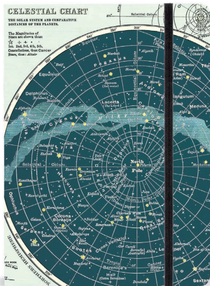
Celestial
