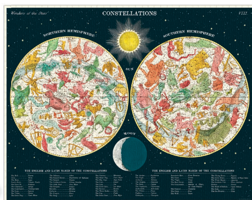
Constellations
