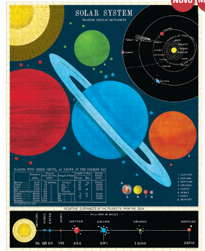
Solar System
