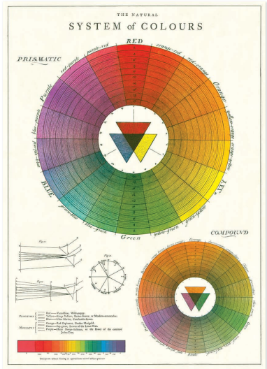
Color Wheel
