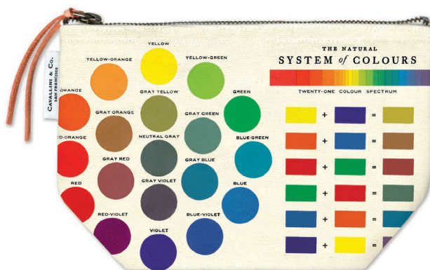
Color Wheel
