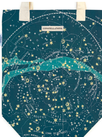
Celestial
