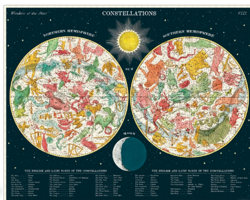
Constellations
