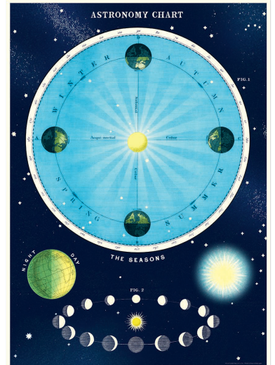
Astronomy Chart
