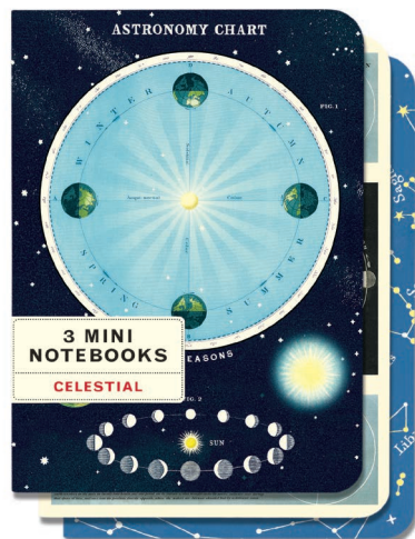
Celestial
