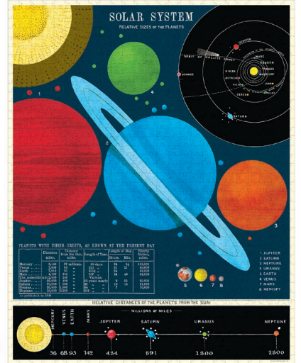
Solar System
