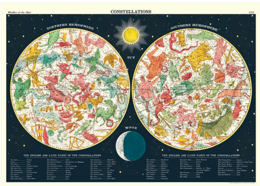
Constellations 2
