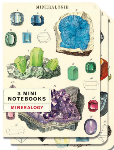
Mineralogy
