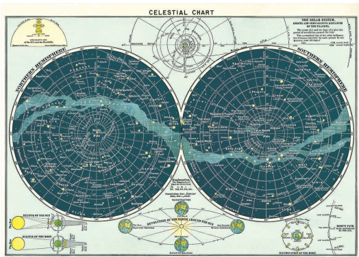
Celestial Chart
