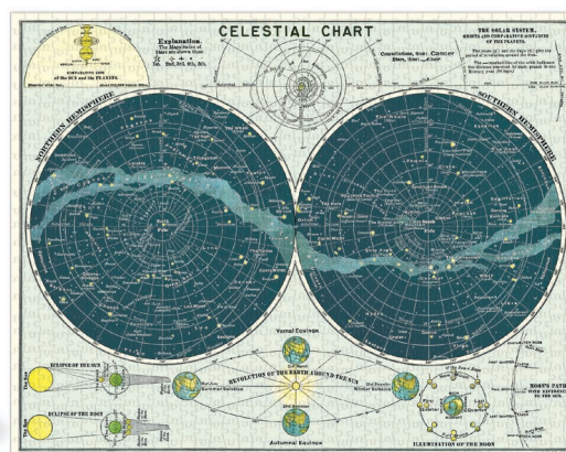
Celestial
