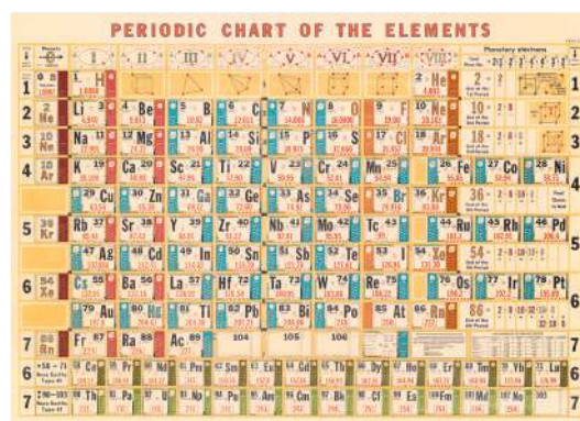
Periodic Chart
