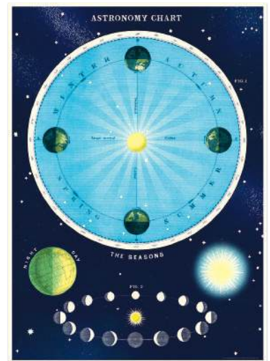
Astronomy Chart
