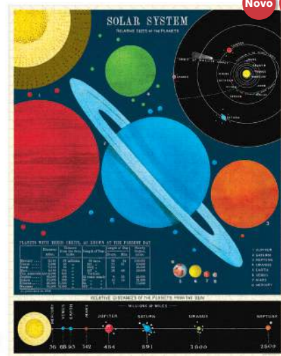
Solar System
