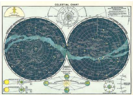
Celestial Chart
