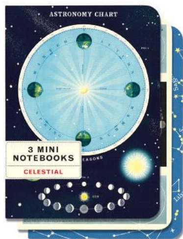
Celestial
