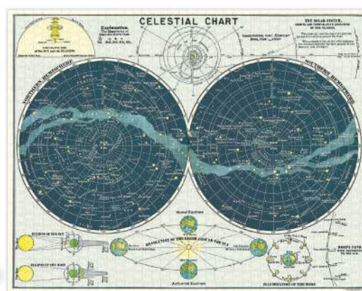
Celestial
