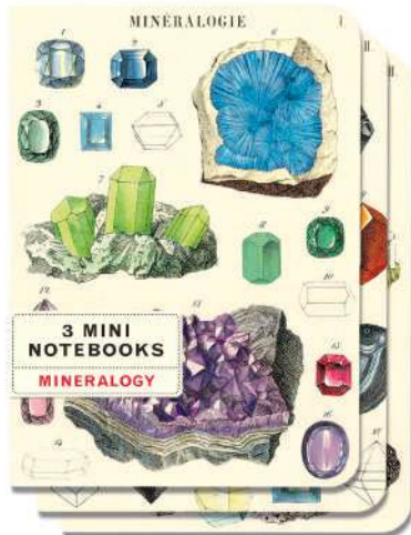
Mineralogy
