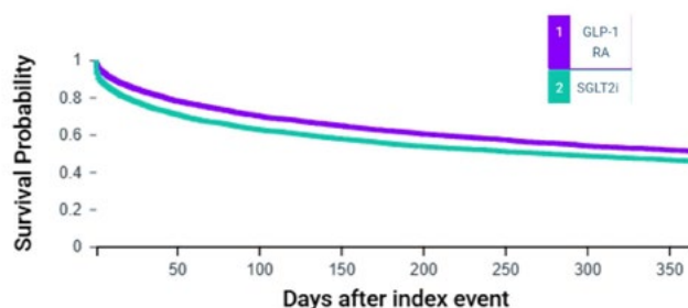
Kaplan-Meier Survival Curve
