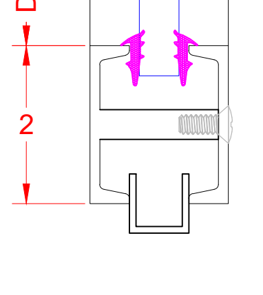
SILL DETAIL
