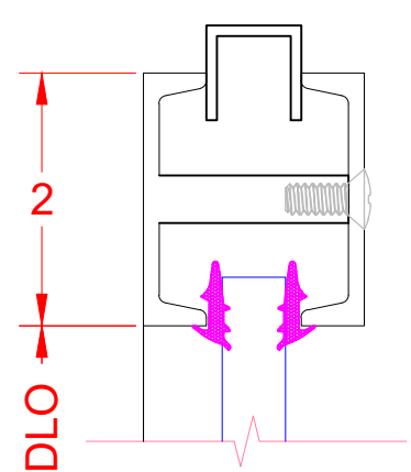
HEAD DETAIL
