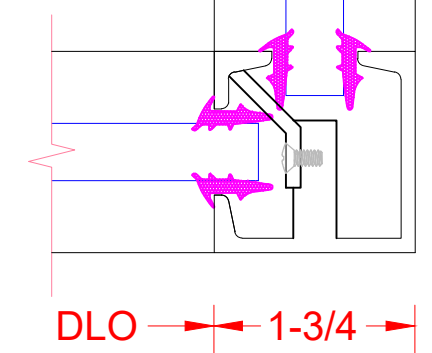
OUTSIDE CORNER DETAIL
