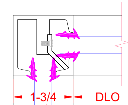
INSIDE CORNER DETAIL
