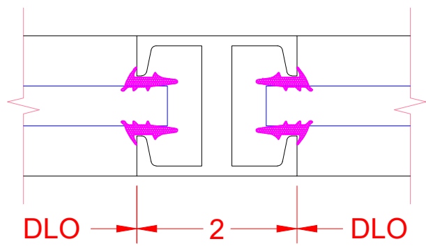
INTERMEDIATE DETAIL
