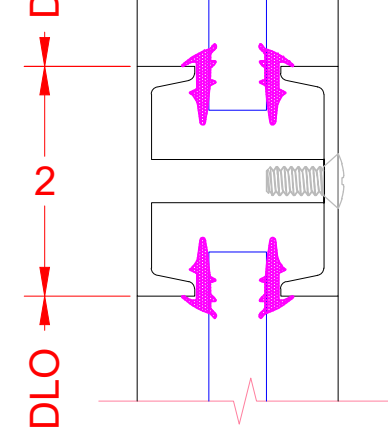
INTERMEDIATE DETAIL
