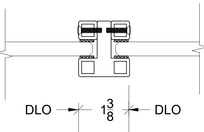
INTERMEDIATE DETAIL
