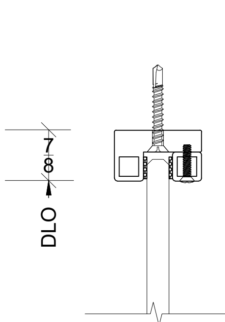
HEAD DETAIL
