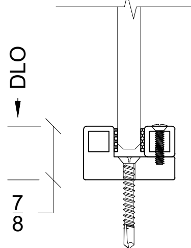
BASE DETAIL
