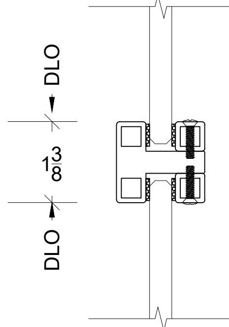
INTERMEDIATE DETAIL
