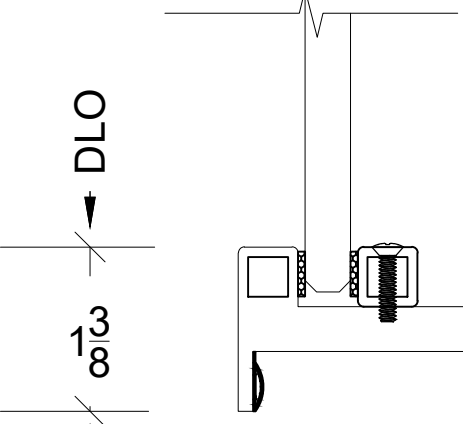
DOOR HEAD DETAIL
