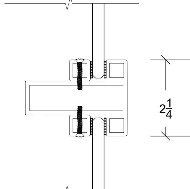
INTERMEDIATE DETAIL
