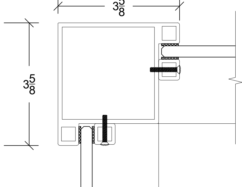
CORNER DETAIL
