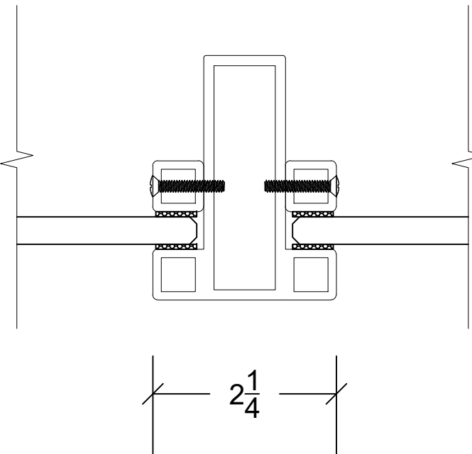
INTERMEDIATE DETAIL
