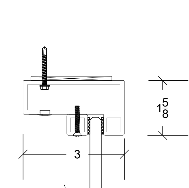
HEAD DETAIL
