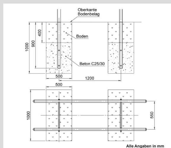
Fundamentplan
