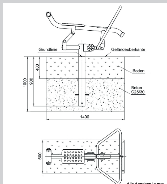
Fundamentplan
