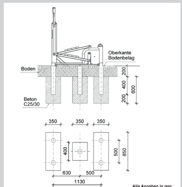
Fundamentplan
