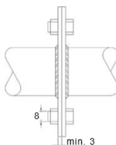
All dimensions in mm Diagram 4.2d
