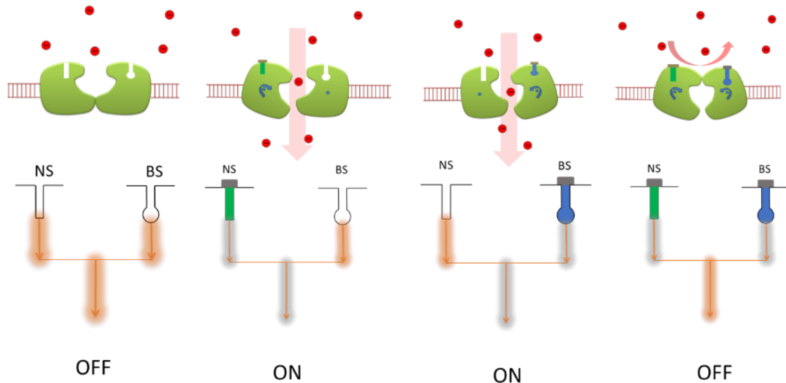
Bivalent chemoreceptor (top) and equivalent EOR logic response for 'single' and 'double' AA binding events
