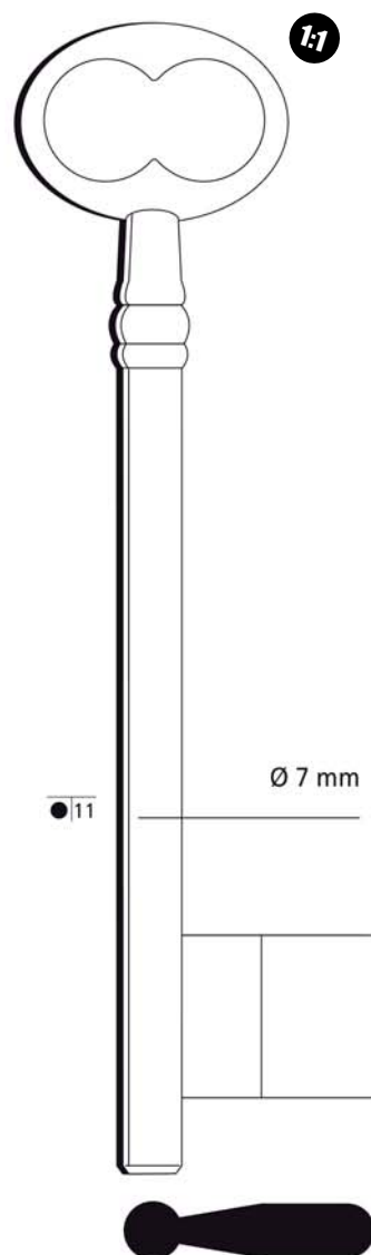
CM1 (in ottone)
