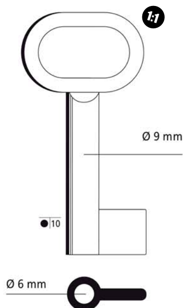
CM2 (in ottone)
