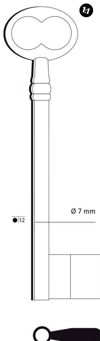
CM2 (in ottone)
