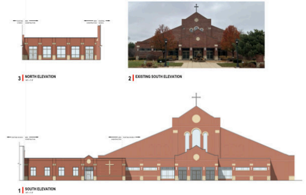
EXTERIOR ELEVATIONS
