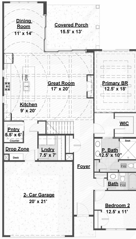
1st Floor
