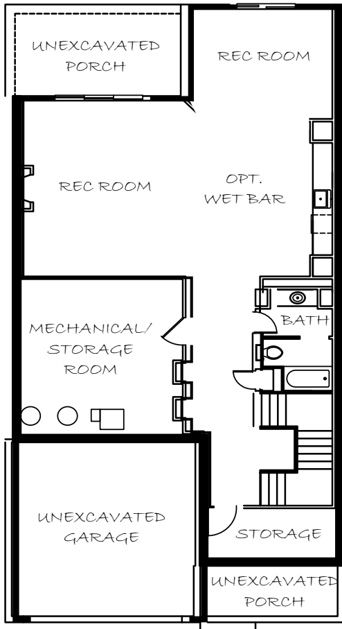
Optional Finished Basement
