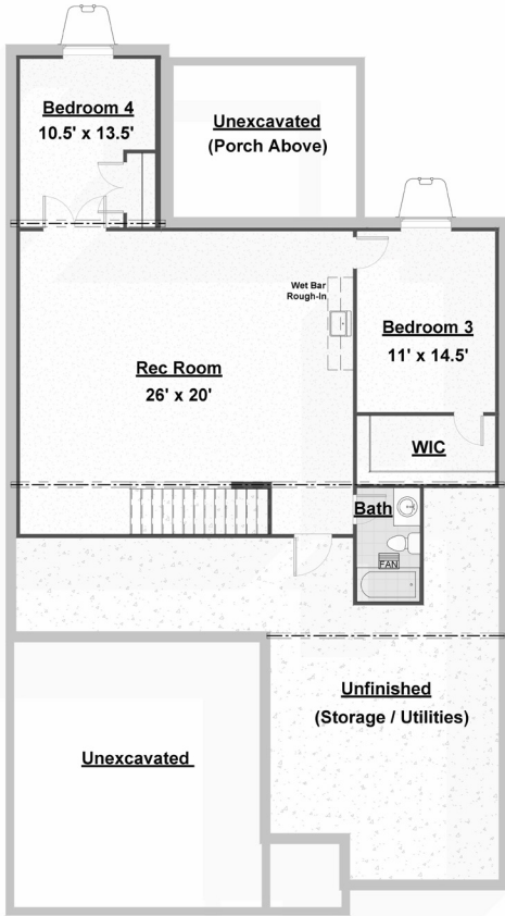
Basement
