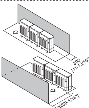
Fig. 12-2-8 Obstacles at rear or front only
