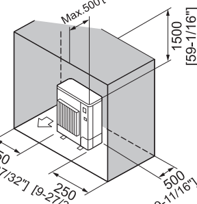
Fig. 12-2-7 Obstacles at rear, sides and above only
