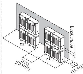
Fig. 12-2-11 Parallel individuals arrangement
