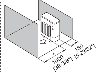
Fig. 12-2-6 Obstacles at front and rear only
