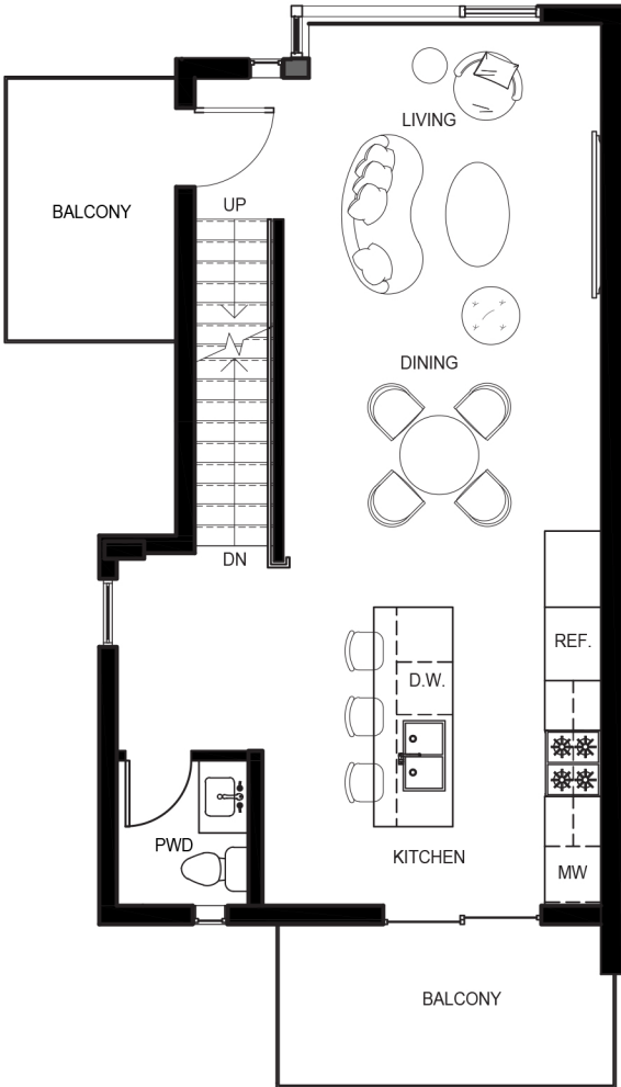
2ND FLOOR
