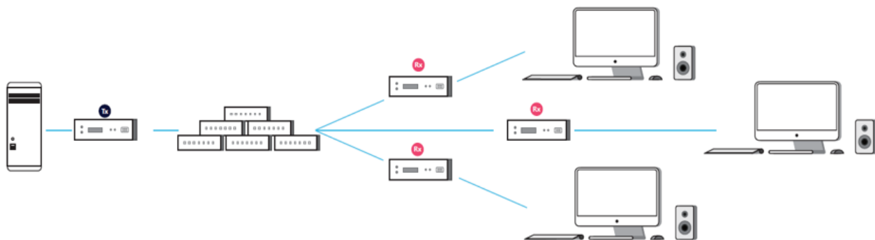
Multiple Rx ends share one source
