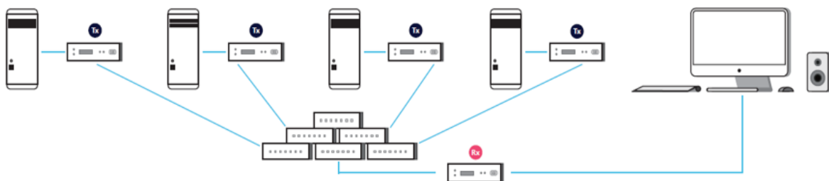
One to multiple sources control, switch on Rx end
