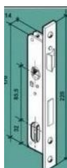
MONTANTE CIL. OVALE ENT. 30/35
