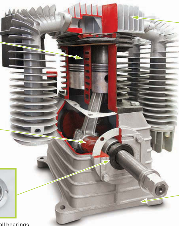
Heavy duty ball bearings for long service
