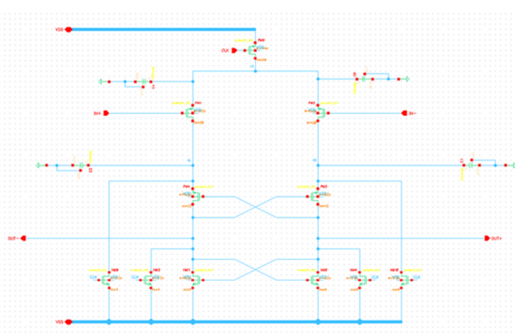
Figure 12 - StrongARM schematic
