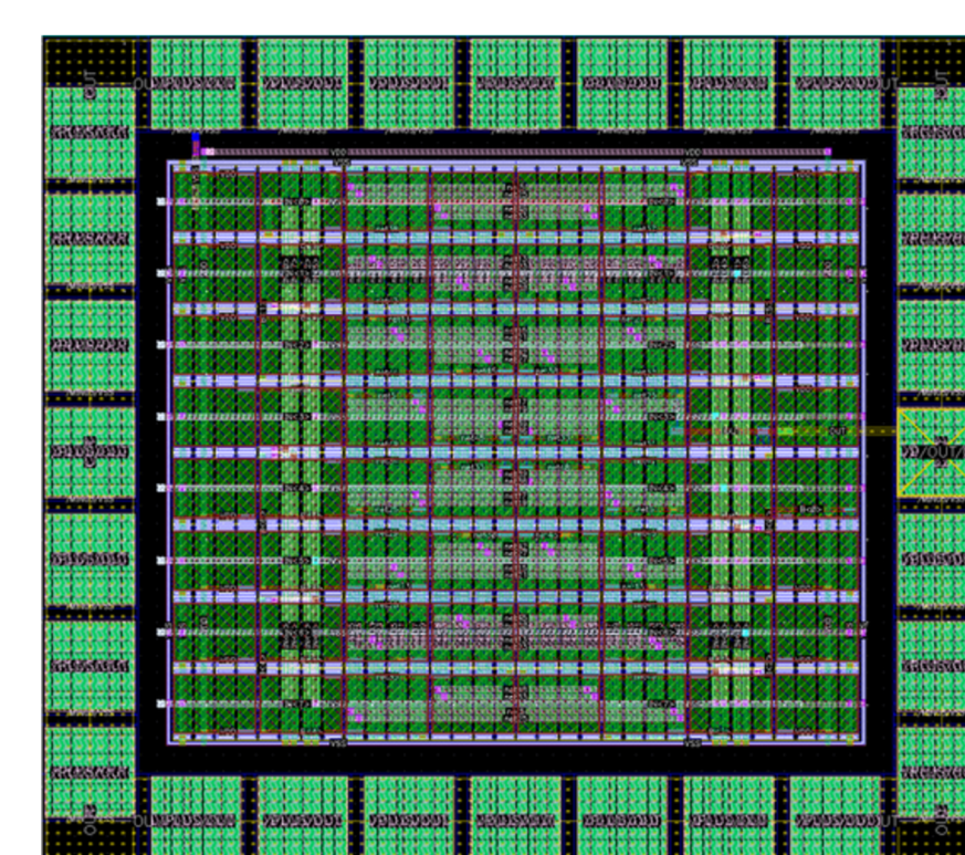
Figure 19 - DAC layout
