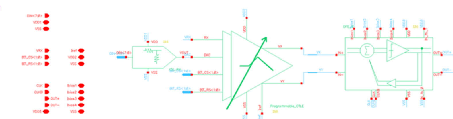
Figure 17 - The final equalizer architecture
