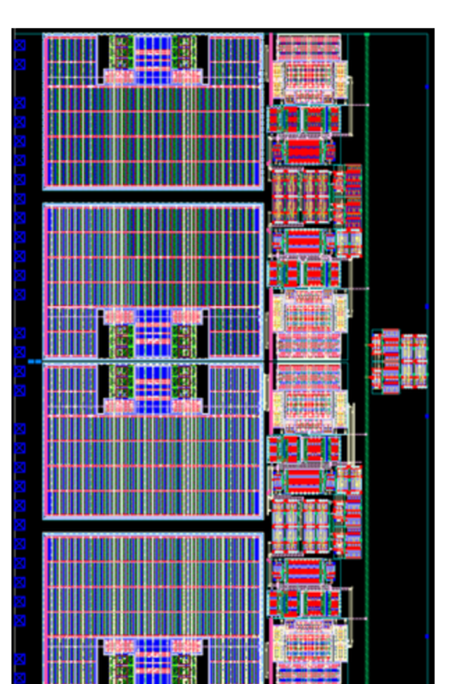
Figure 21 - DFE layout
