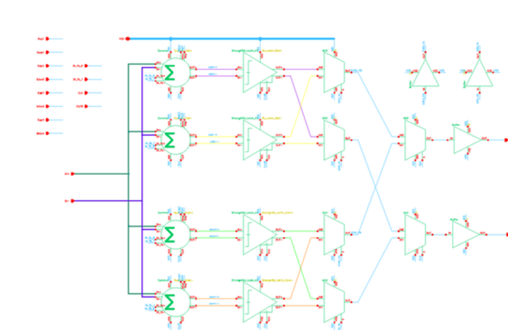
Figure 15 - Loop-Unrolled DFE Architecture
