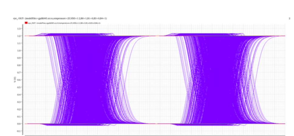
Figure 23 - Post-layout eye diagram
