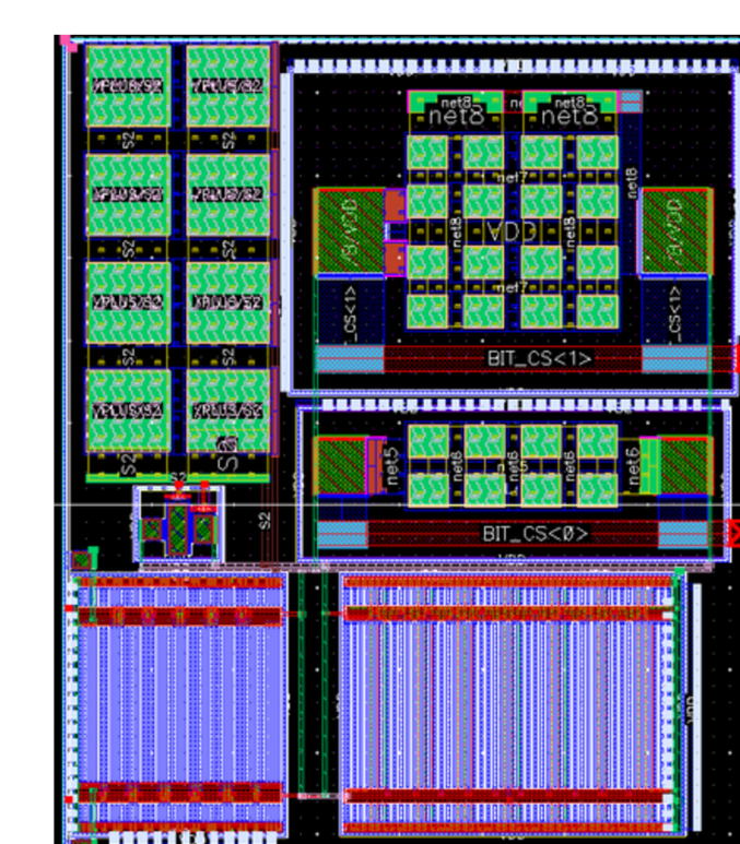
Figure 20 - CTLE layout
