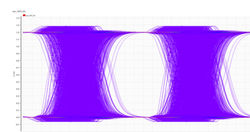
Figure 22 - Pre-layout eye diagram
