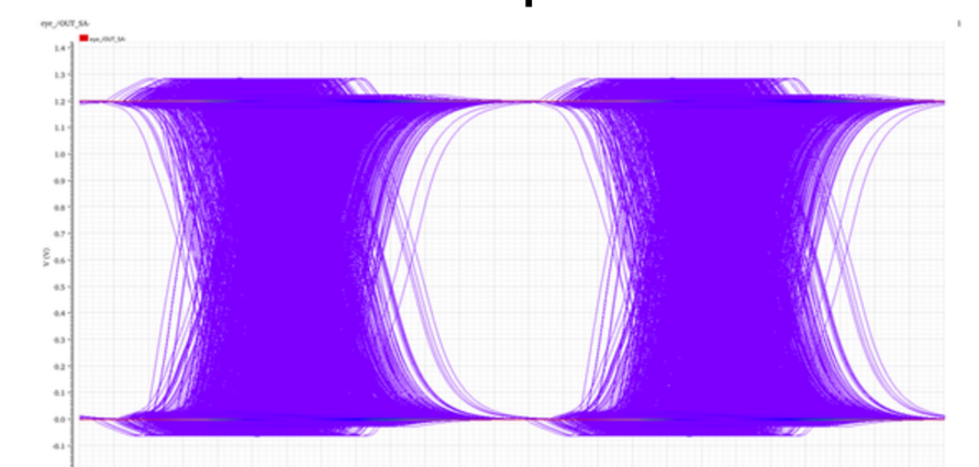
Figure 18 - The full system eye diagram
