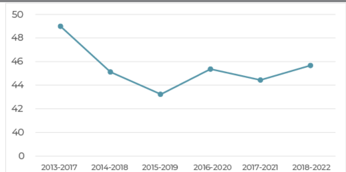
Figure 2.10: Nonmotorized Crashes
