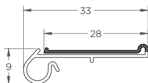
RT-037 (Portaprecio Blister 30 mm )
