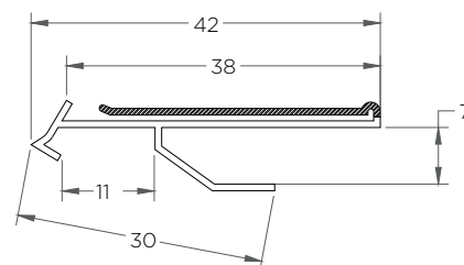
RT-036 (Portaprecio enganche central 40mm bicolor)
