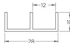
PT-012 (Carrilera 28 mm PS)
