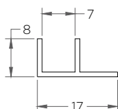
RT-031 (F 17 mm)
