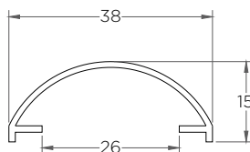
ET-023 (Bomper PVC Blando)
