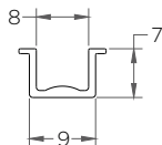
RT-023 (U closet)
