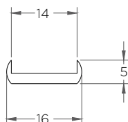
BT-009 (Cinta borde curvo 14 mm)
