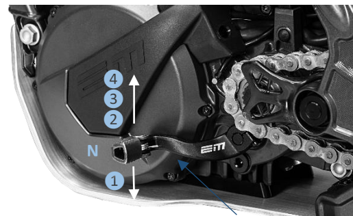
Gearshift pedal
