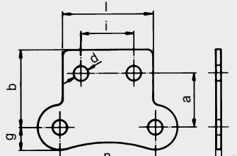
Design 101.2 for double-pitch chains
