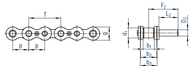
Type F extended pins (available on alternate sides)
