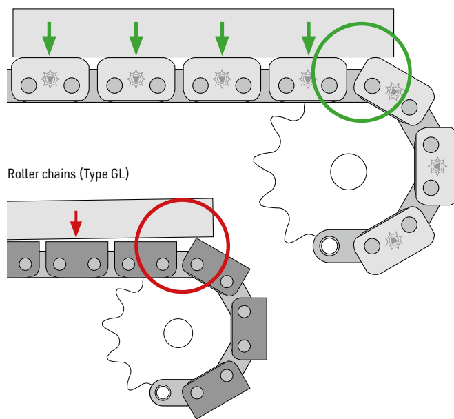
Roller chains (Type GL) with POM-Clip
