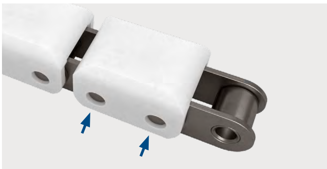
Fixing by pin extensions, chains preferably unriveted
