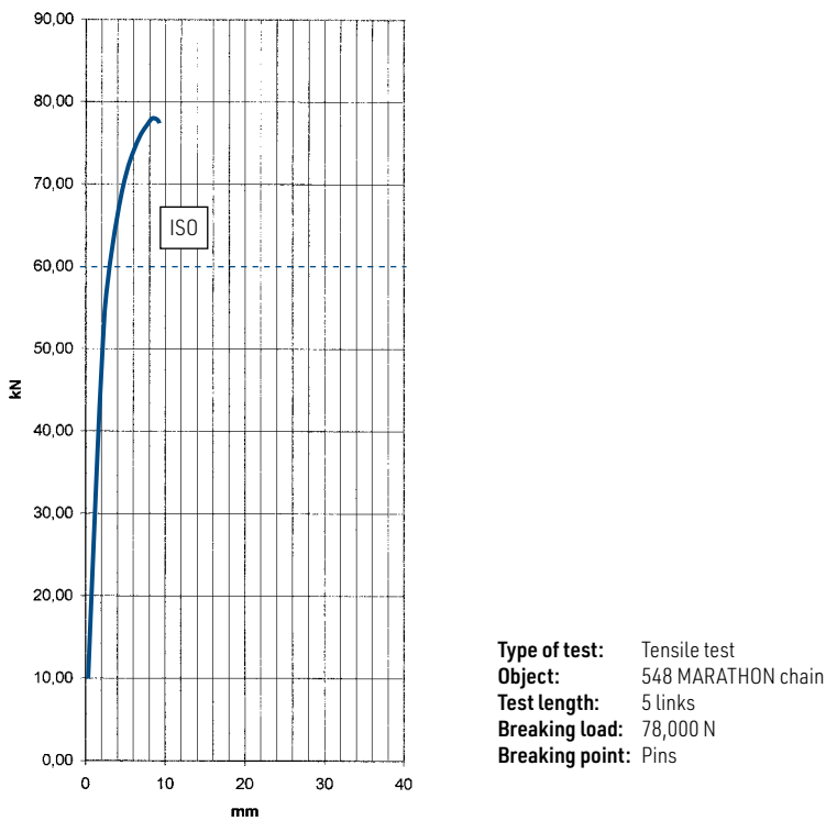
Force projection diagram
