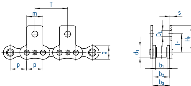
Type E straight attachments, both sides
