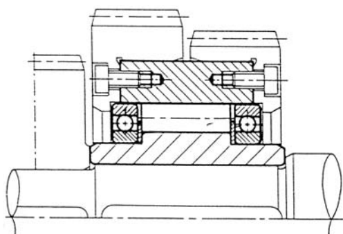
GFR-K in a transmission
