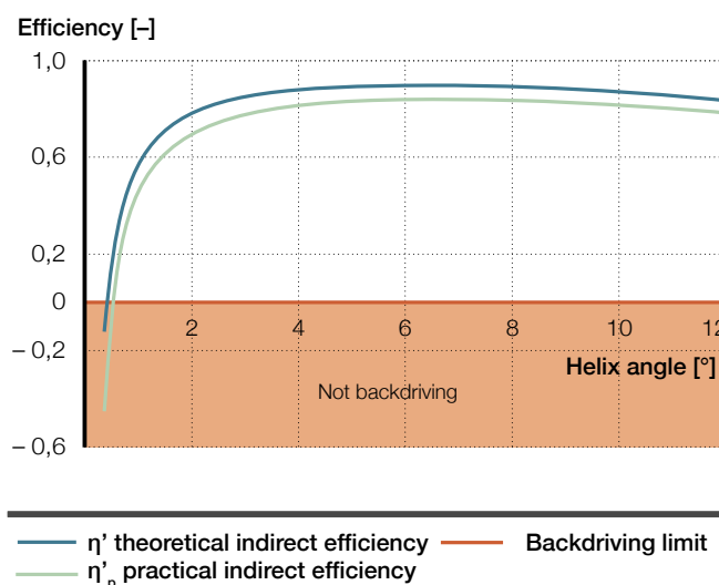
Theoretical and practical indirect efficiency
