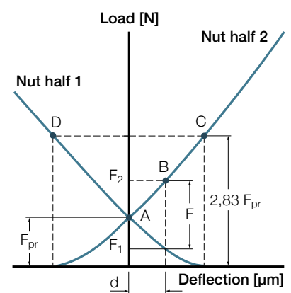
Fig. 8 Concept of preloaded nut
