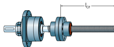
Fig. 25 Mounting factor f_1 = 0,9
