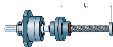
Fig. 27 Mounting factor f_1 = 3,8
