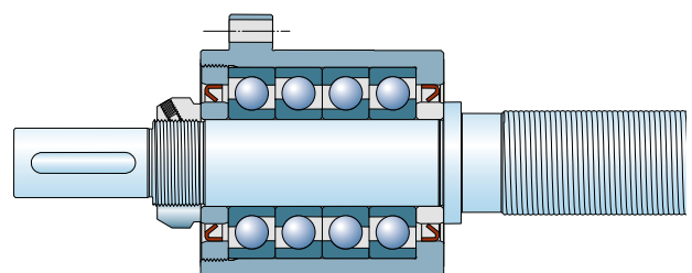
Support bearing assembly
