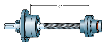
Fig. 28 Mounting factor f_1 = 5,6
