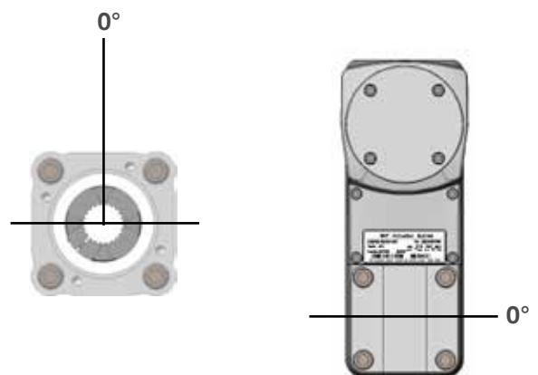
Gearbox orientation
