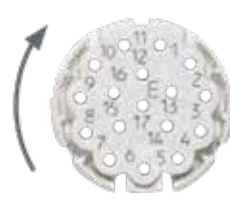
Intercontec AEDC 139 NN 00 00 1215 000 (insert at 0°)
