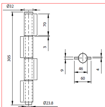
MAXI CERNIERA A 4 ALI
