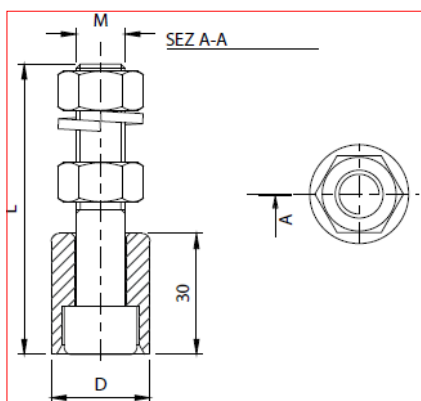
OLIVA A RULLO IN NYLON BULLONE ZINCATO
