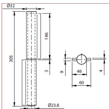
MAXI CERNIERA A 2 ALI
