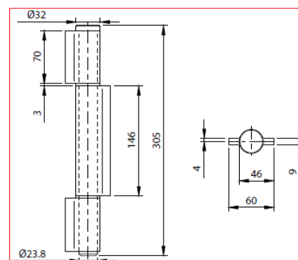
MAXI CERNIERA A 3 ALI
