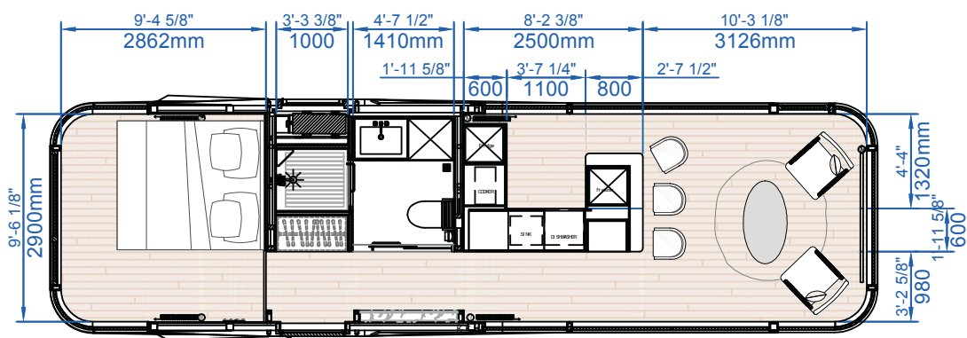
INDOOR PLAN VIEW
