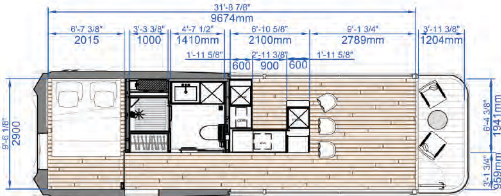
INDOOR PLAN VIEW
