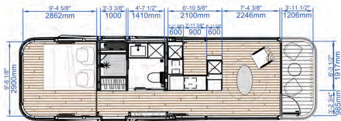
INDOOR PLAN VIEW
