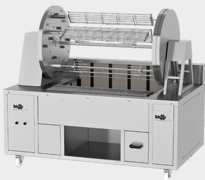
Multi Spit Roasting Machine with 12 Rotating Spit Positions & Rotating Wheels
