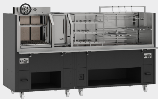
Customised Super 475- Combination Parrilla Grill, Fire Box, Rotisserie, Cantilever Grilling Station with Spit & Hanging Rails
