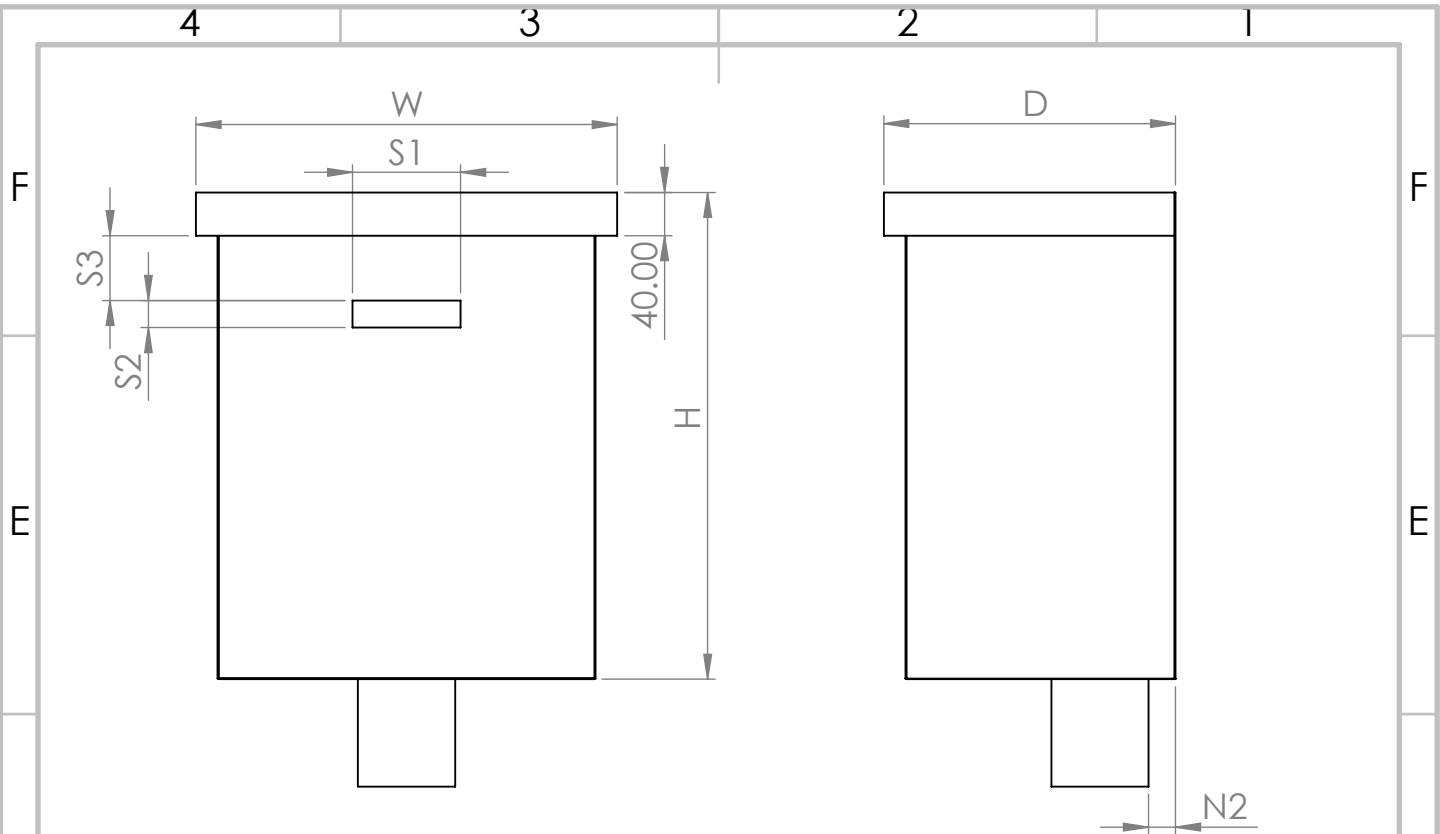
FRONT VIEW
