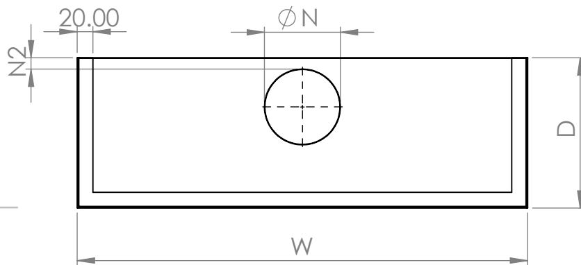
PLAN VIEW
