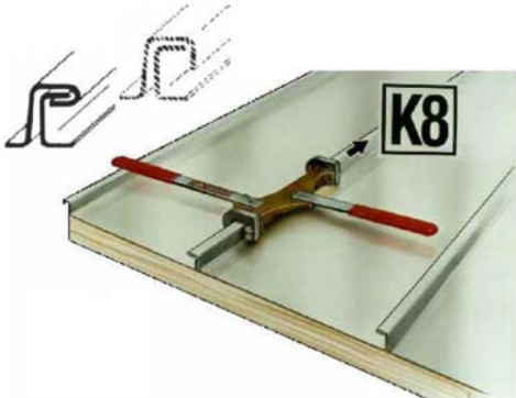
SINGLE LOCK SEAMER
