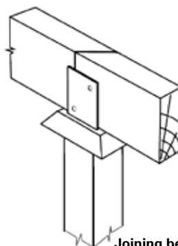
Joining bearers on Pier
