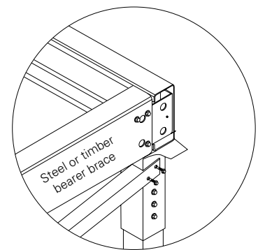
Steel or timber bearer
