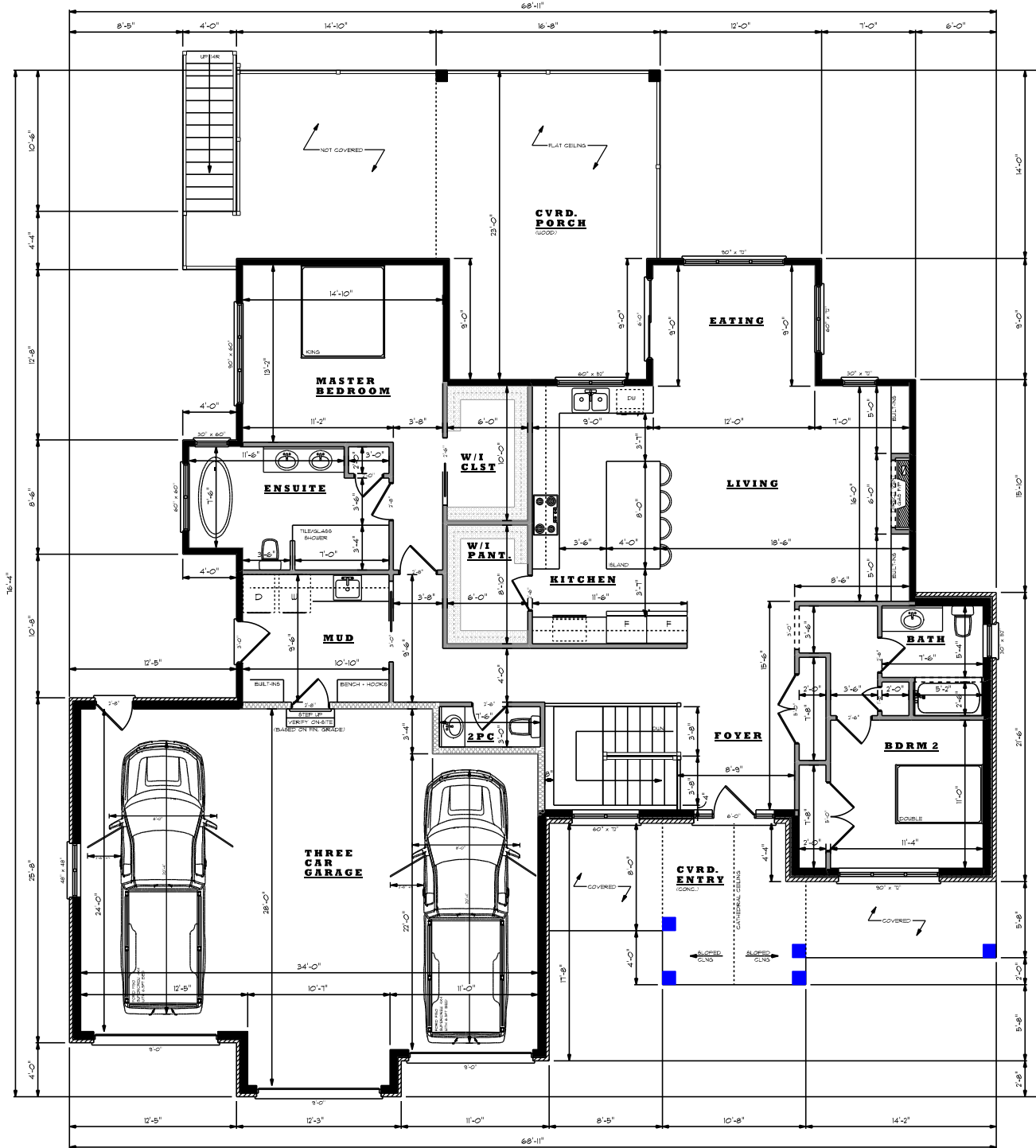
MAIN FLOOR PLAN "F" (NOT FOR CONSTRUCTION) Not to scale S:\Projects\COUNTY HOMES\302 Michael's Way\ February-22-24 Square Footage: 1966.5 sq. ft. Client's Email: Rijus Home Design Inc www.rijus.com Jason Schilstra (CH) 905-701-1110
