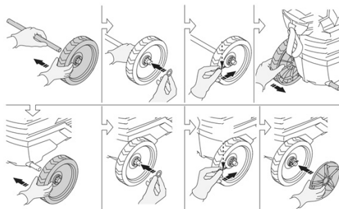
Fig. 3 – Instalando as rodas
