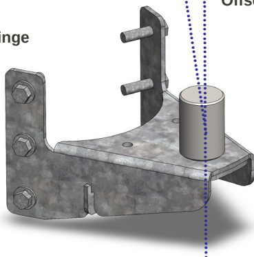
Offset Gudgeon
