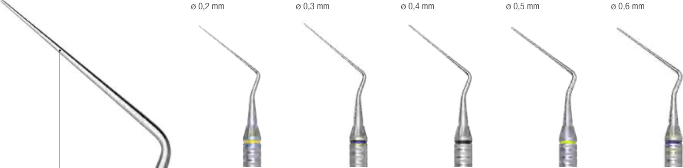
543/1.C6 ISO 20 Yellow Giallo 543/2.C6 ISO 30 Blue Blu 543/3.C6 ISO 40 Black Nero 543/4.C6 ISO 50 Yellow Giallo 543/5.C6 ISO 60 Blue Blu
