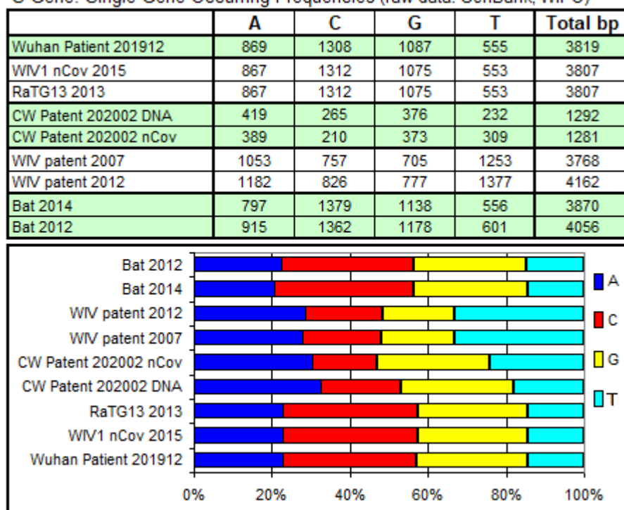
S-Gene: Single Gene Occurring Frequencies (raw data: GenBank, WIPO)
