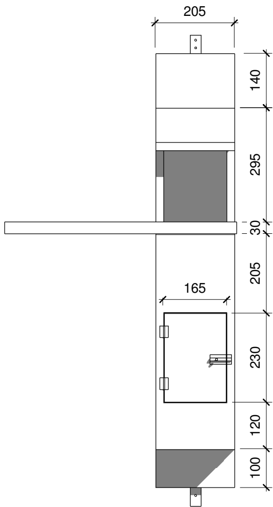
Front Elevation
