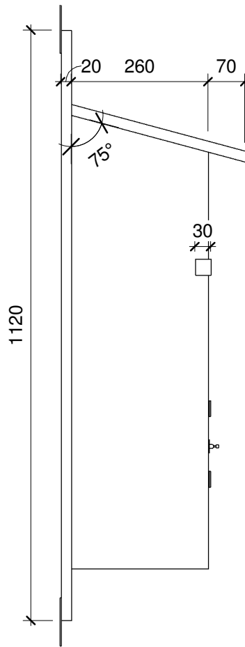
Side Elevation
