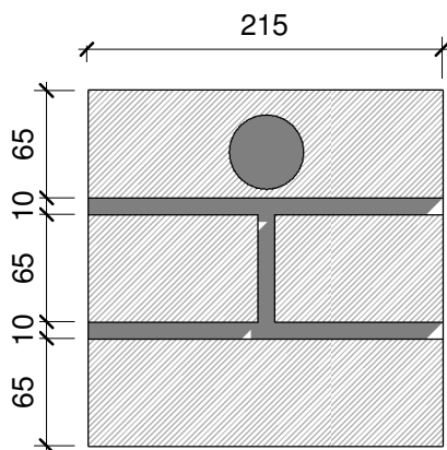
Front Elevation
