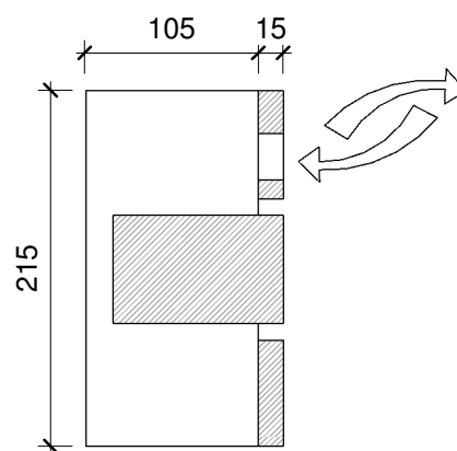
Side Elevation
