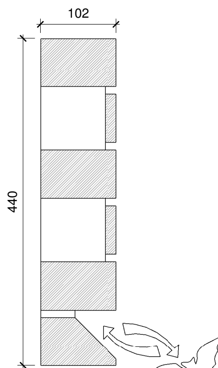
Side Elevation
