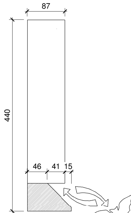
Side Elevation
